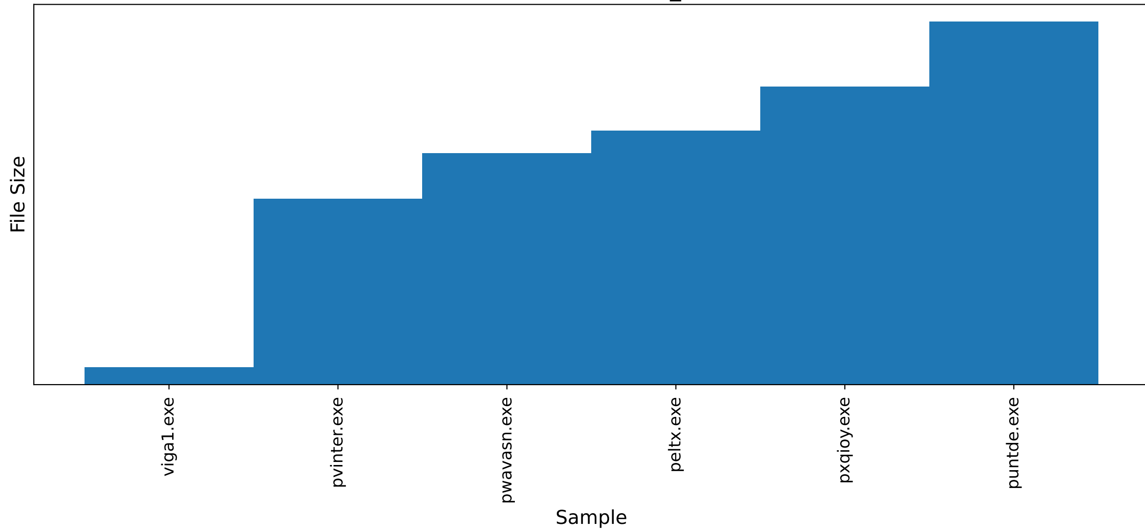
Size distribution of Cluster25_Size6 dataset
